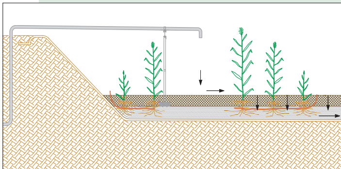
Cross Section of a PURE-Plant
