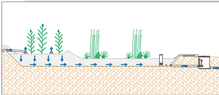
Biological Treatment
